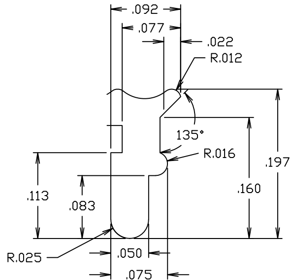
8X FULL SIZE DETAIL "B"
